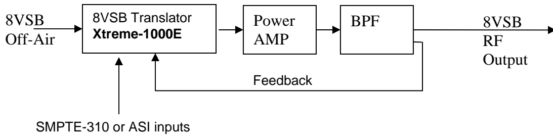
Figure 4: Application of the XTREME-1000E for 8VSB Digital Translator
