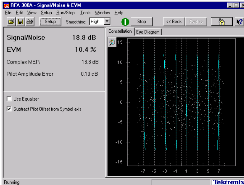
Figure 7.1 SNR measurement before linear precorrection
