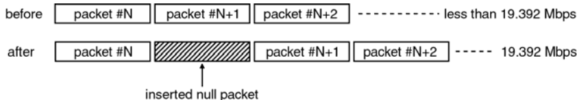
Figure 1-2: Null Packet Insertion
